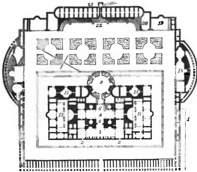
FIG. 5.—Ground plan of the baths of Caracalla.
