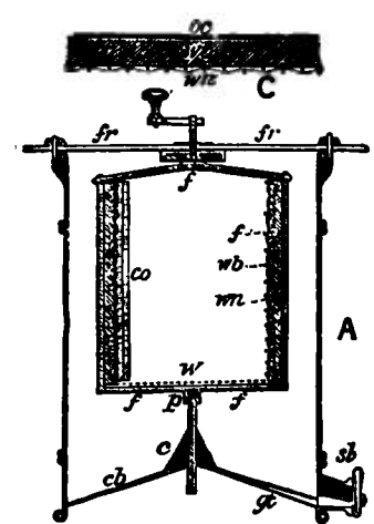
FIG. 19.—Diagram of the Raynor Extractor.
