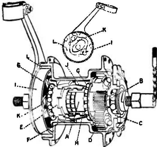
FIG. 12.—Eadie Two-speed Coaster Hub.
