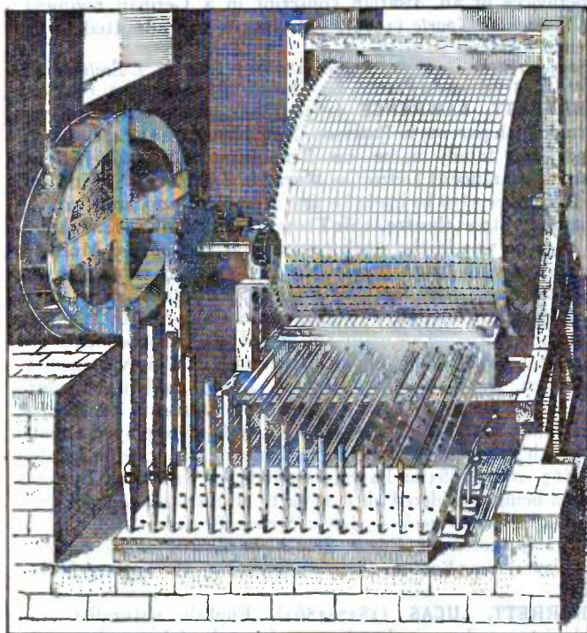
FIG. 1.—Large stationary barrel-organ worked by hydraulic power, from Solomon de Caus, Les Raisons des forces mouvantes (Frankfort-on-Main, 1615).
