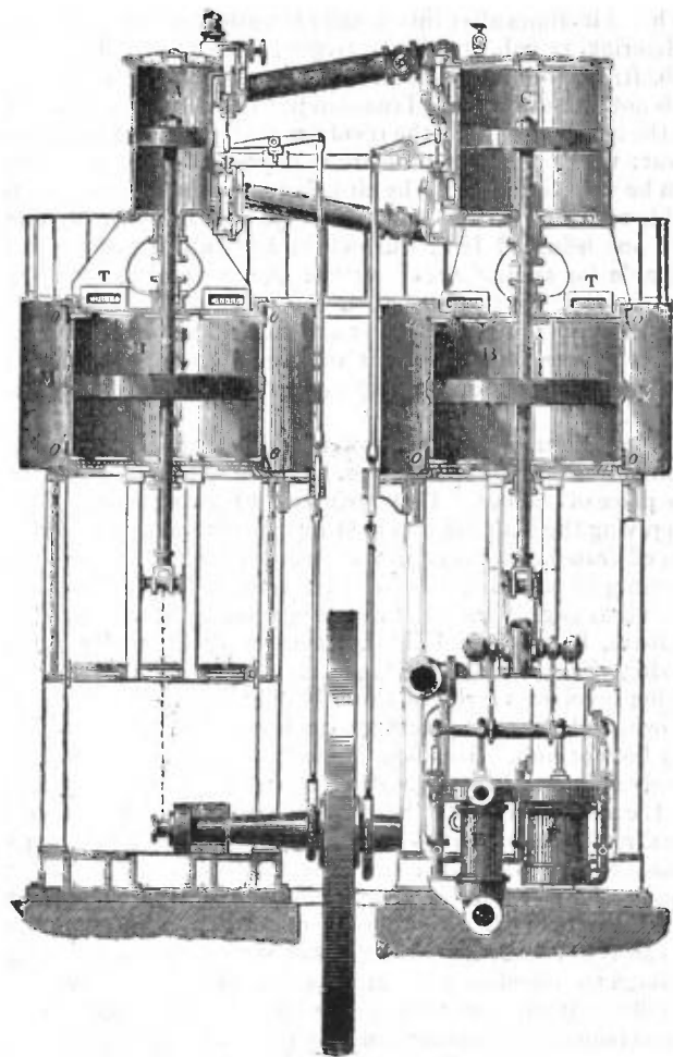
FIG. 4.—Vertical Section of Lackenby Blowing Engines (1871).
