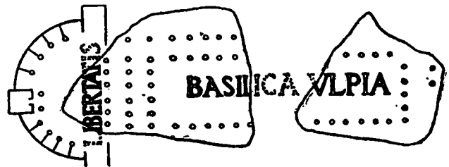
FIG. 3.—Plan of Basilica Ulpia, from Capitoline plan of Rome.
