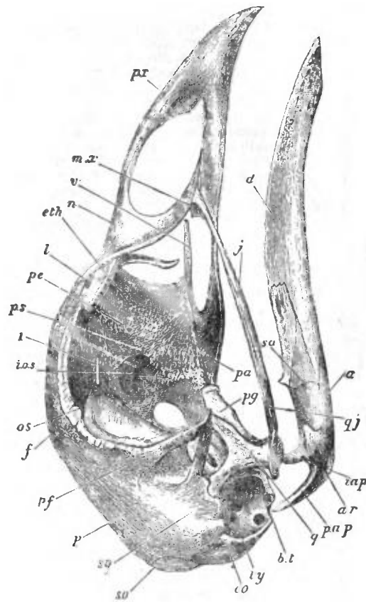
FIG. 6.—Skull of adult Fowl. Here the temporal fossa is bridged over by the junction of the post-frontal and squamosal processes ( pf , sq ). The processes of the mandible ( iap , pap ) are characteristic of this type, and of the anseres.
