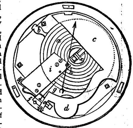
FIG. 4.—Aneroid Barometer.
