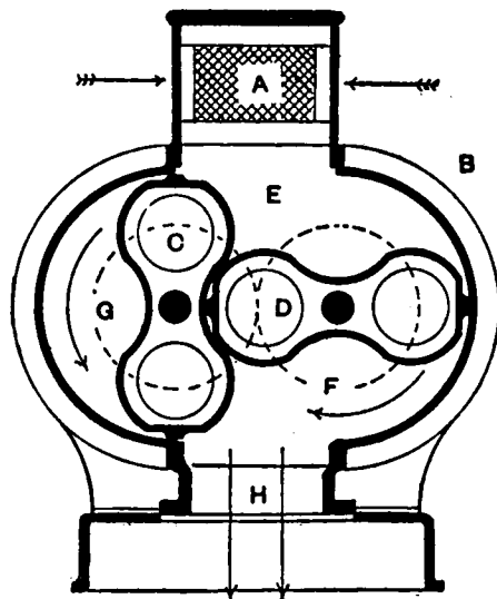
FIG. 6.—Thwaites' Improved Roots' Blower.
