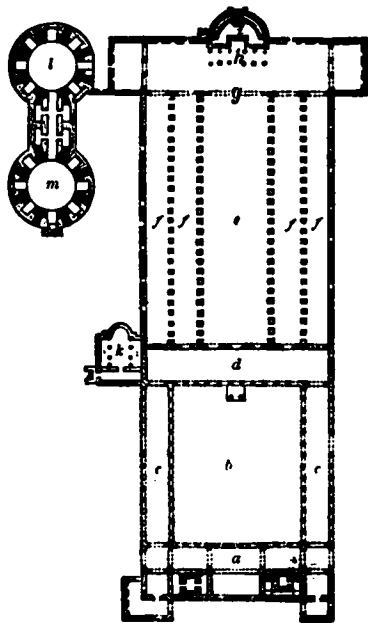
FIG. 10.—Ground-Plan of the original Basilica of St Peter's at Rome. a , Porch. b , Atrium. c , Cloisters. d , Narthex. e , Nave. f, f , Aisles. g , Bema. h , Altar, protected by a double screen. i , Bishop's throne in centre of the apse. k , Sacristy. l , Tomb of Honorius. m , Church of St Andrew.
