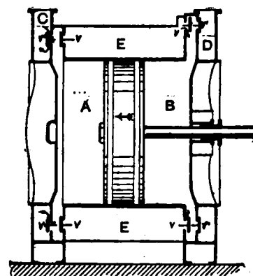
FIG. 5.—Richardsons, Westgarth & Co.'s Blowing Engine.
