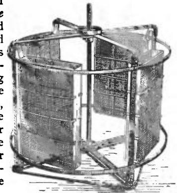
FIG. 21.—Cowan's four-frame Extractor; interior.
